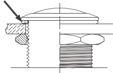
O型防水圈 O-type waterproof ring
